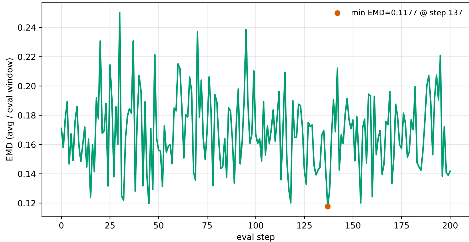
EMD over training — Quantum V2 (135p)
