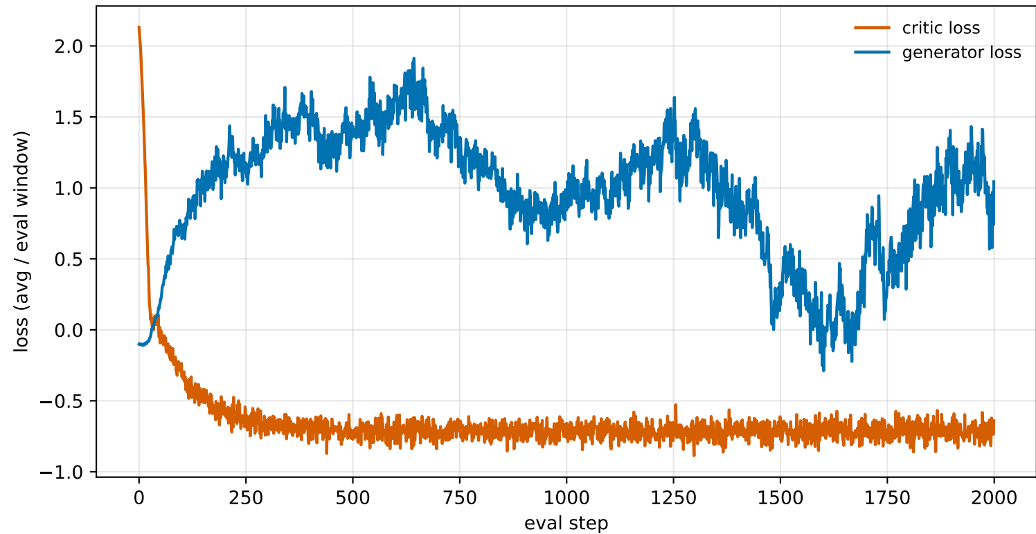
Training/fit curve — WGAN-GP (LSTM)
