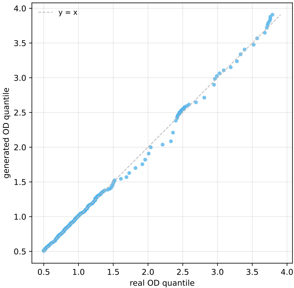
Q-Q plot — Quantum V1 (75p)
