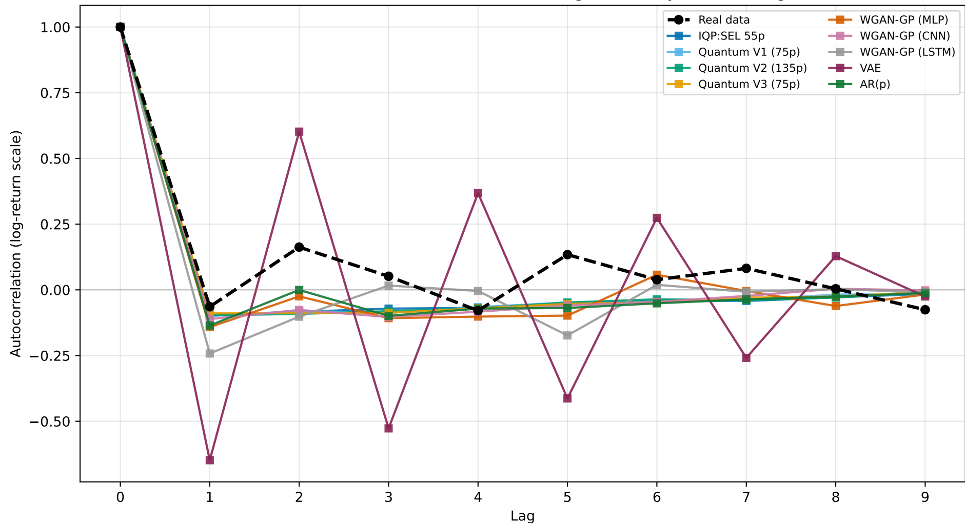
Cross-model log-return ACF overlay — matched 2000-epoch budget, mean over 5 seeds (real-data reference: dashed black; VAE lag-1 anomaly visible at lag=1)
