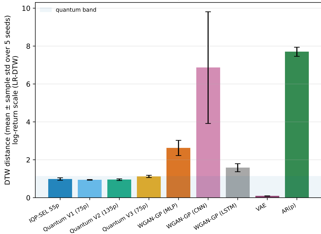
Cross-model DTW — log-return scale (LR-DTW)
