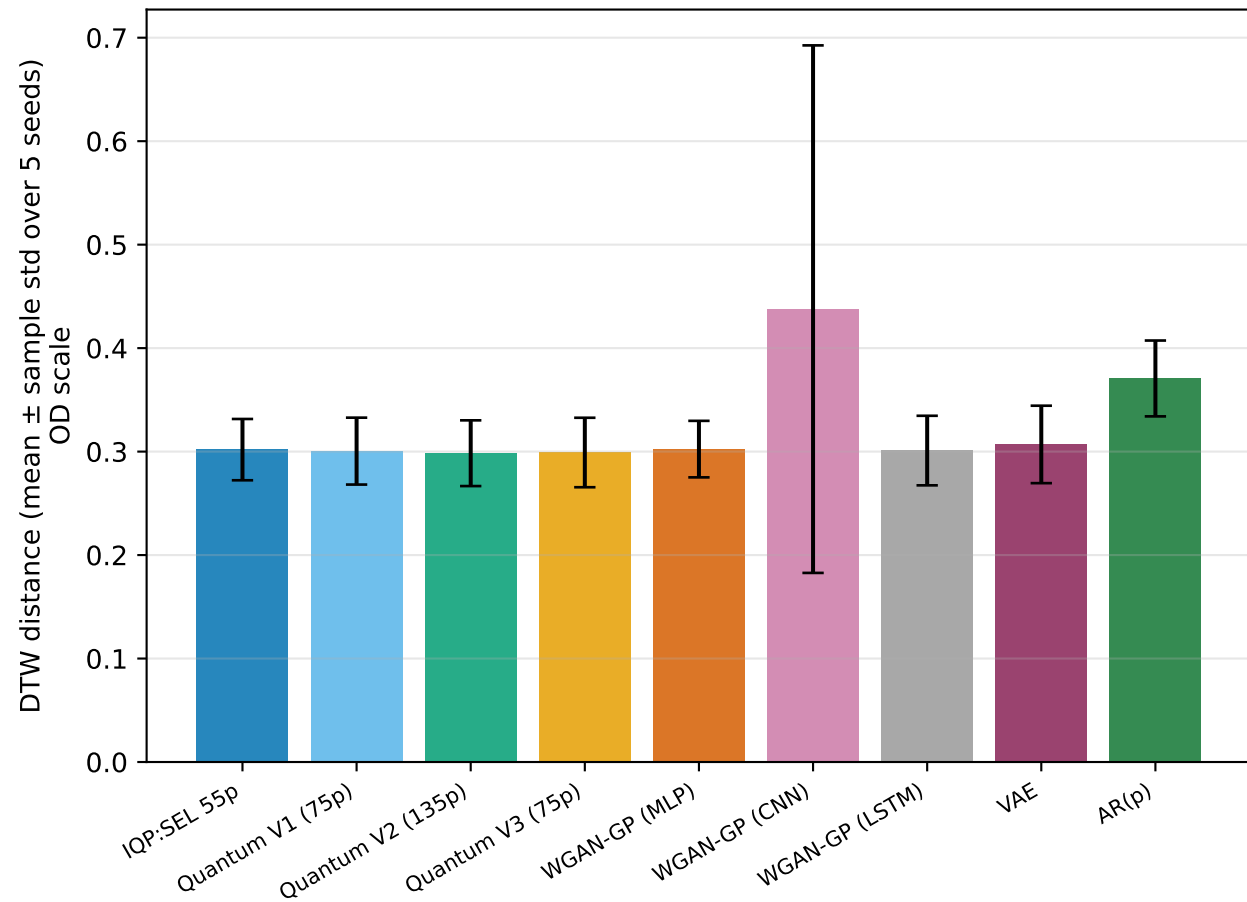
Cross-model DTW — OD scale
