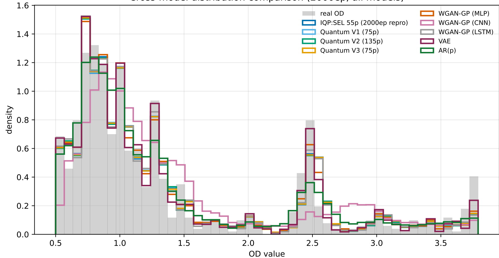
Cross-model distribution comparison (2000ep, all models)
