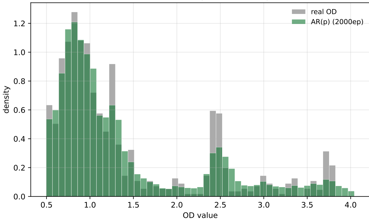
Distribution comparison — AR(p)
