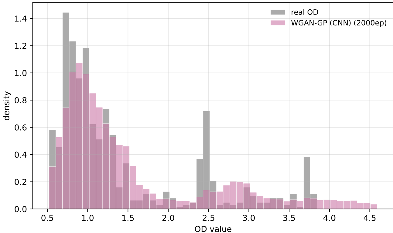
Distribution comparison — WGAN-GP (CNN)
