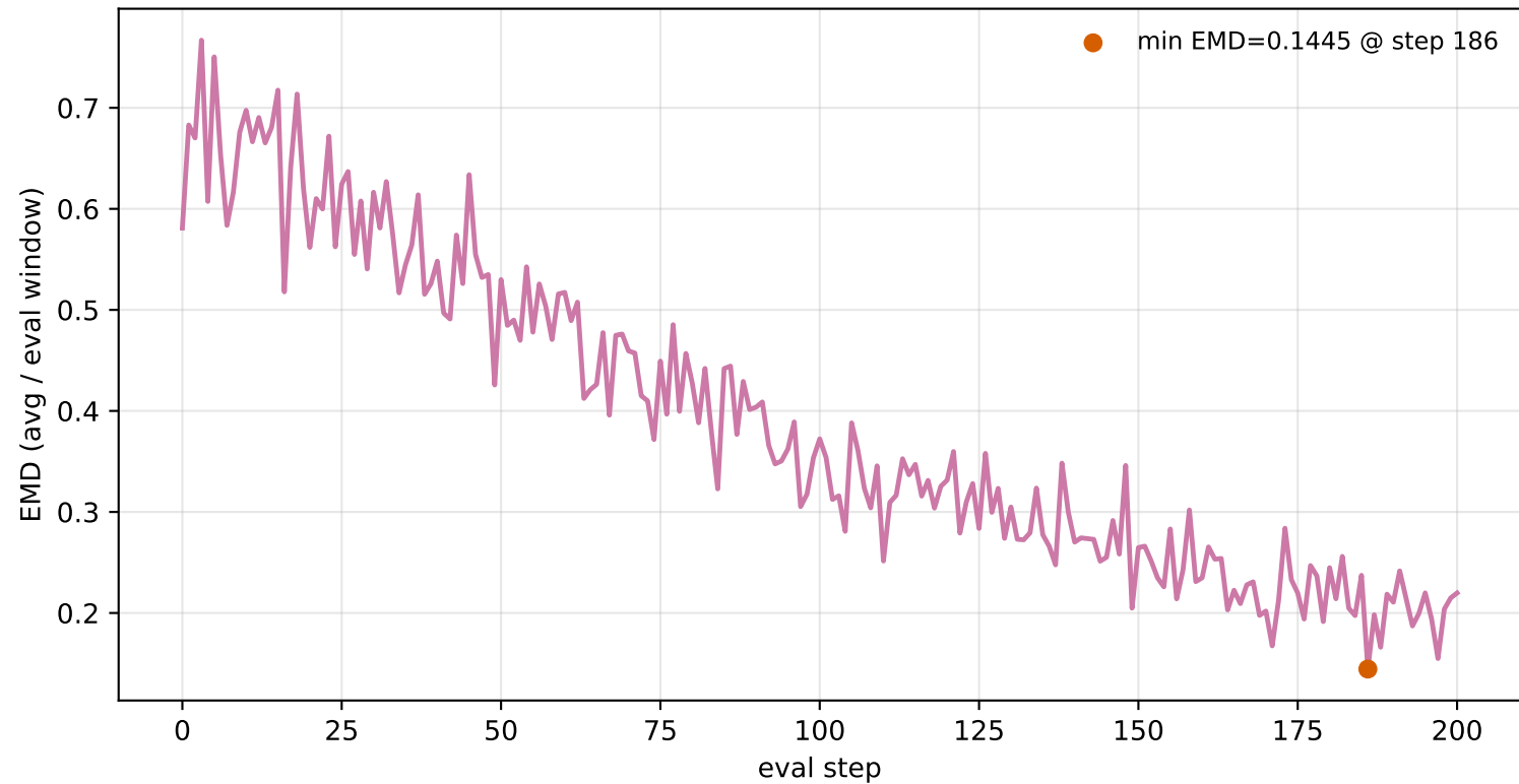
EMD over training — WGAN-GP (CNN)
