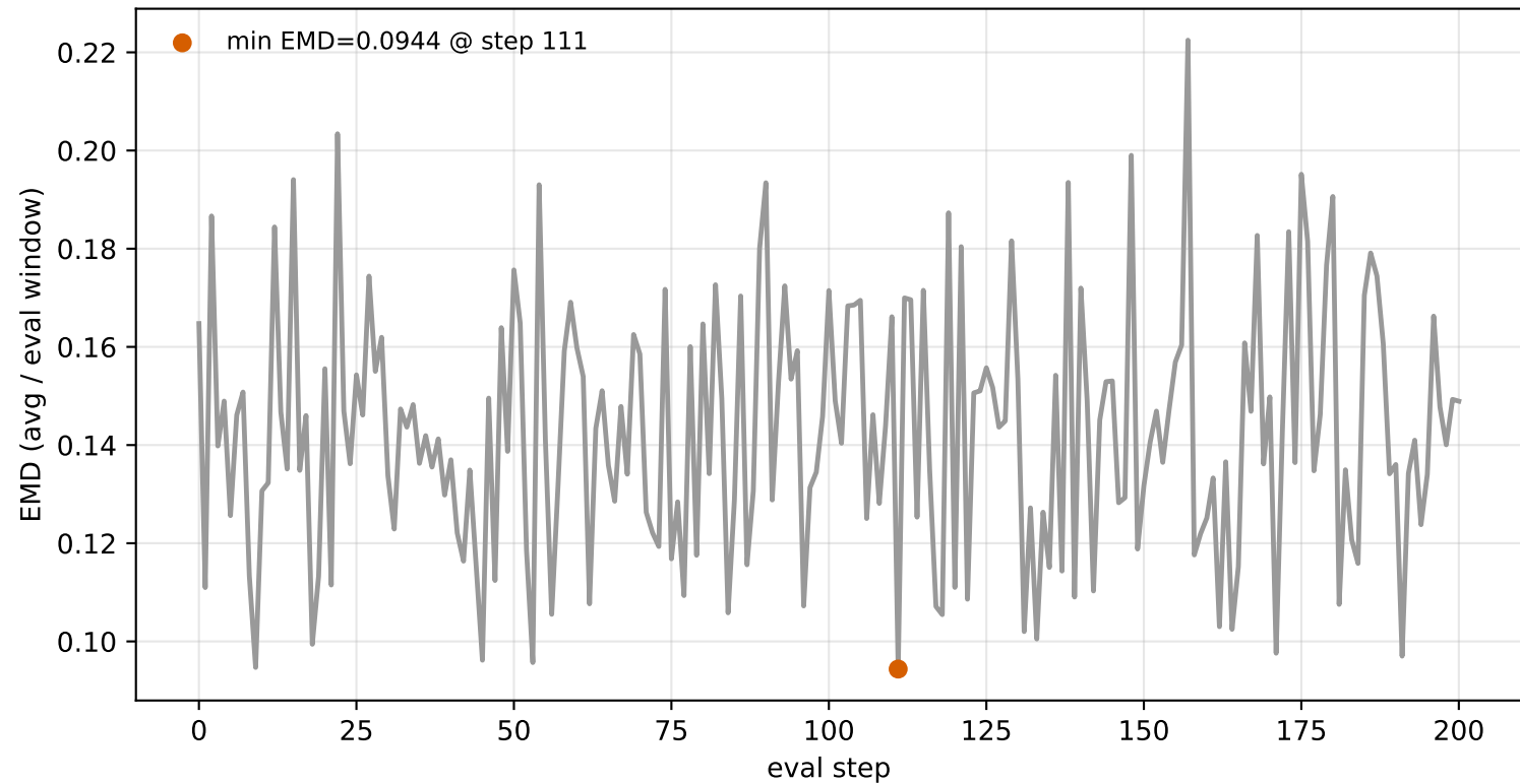
EMD over training — WGAN-GP (LSTM)
