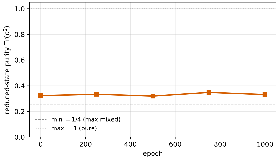
(b) State purity vs epoch
