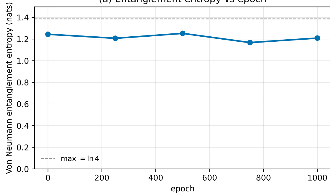
(a) Entanglement entropy vs epoch
