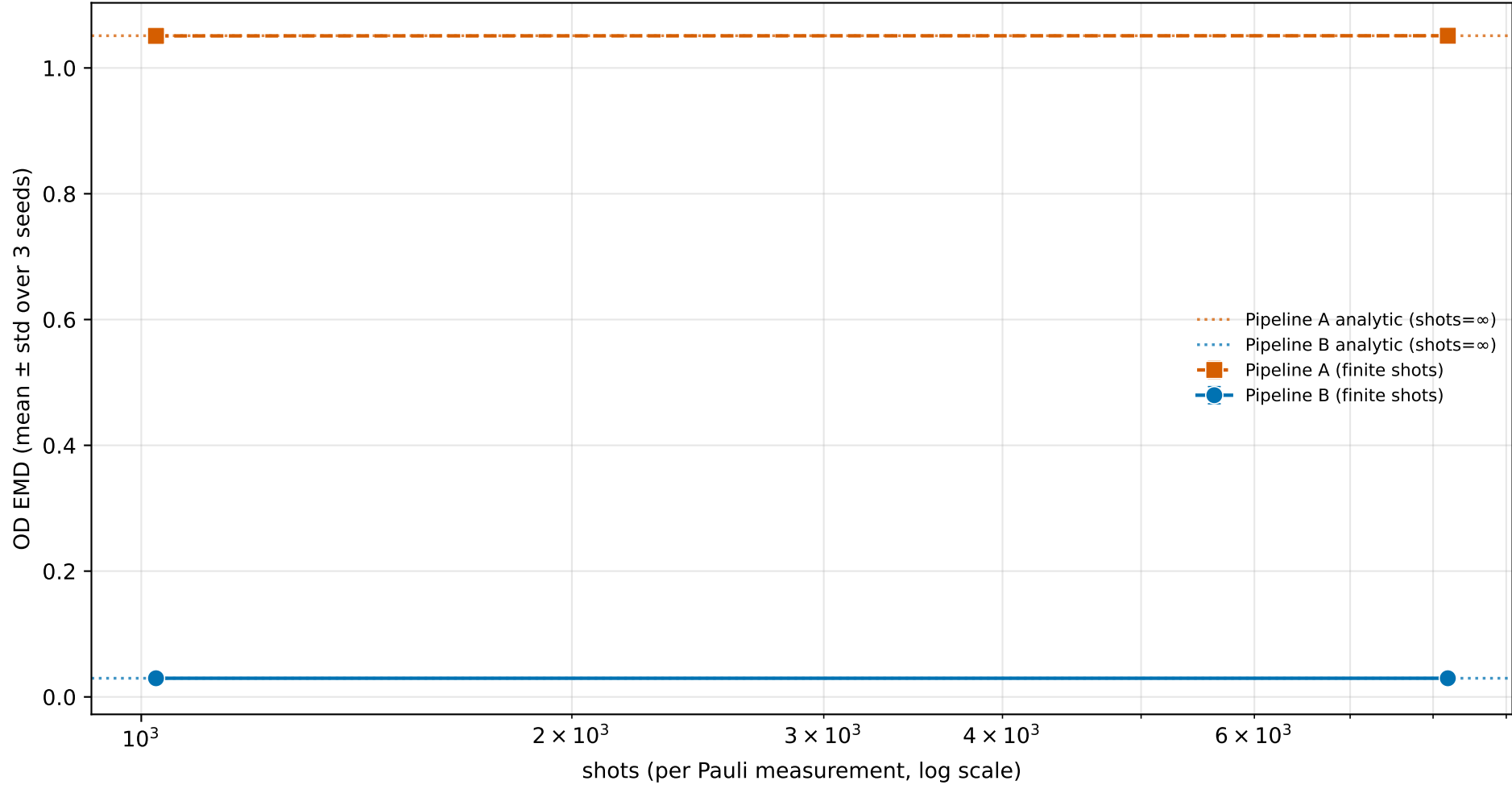
Shot-noise robustness — EMD vs shot count (log-x). Analytic-statevector baseline (shots= \infty ) shown as horizontal reference per pipeline. Mean over 3 seeds (42-44); error bars are seed std.
