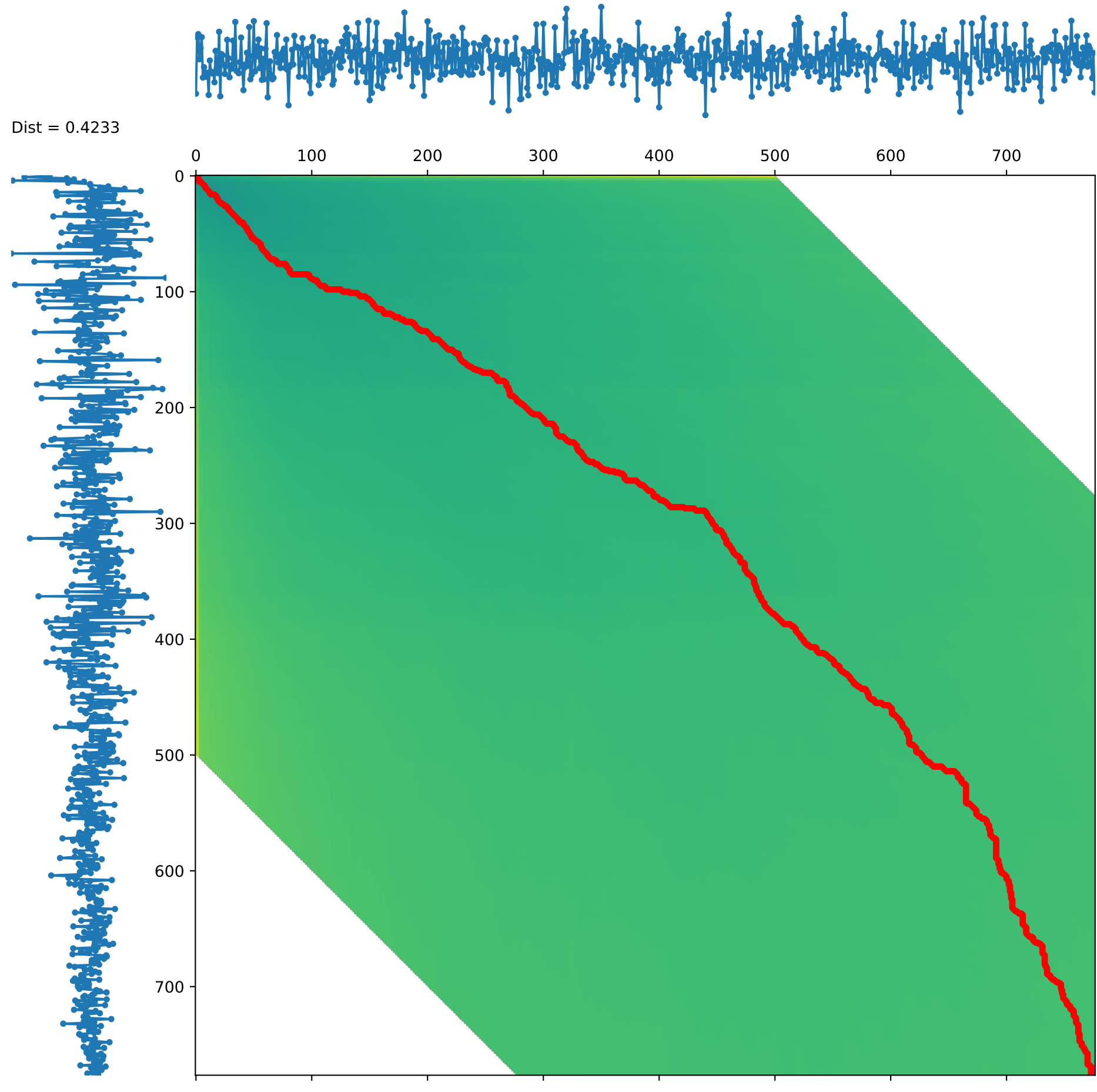
DTW alignment — IQP:SEL 55p (2000ep repro) (seed 42, window=500, psi=2)
