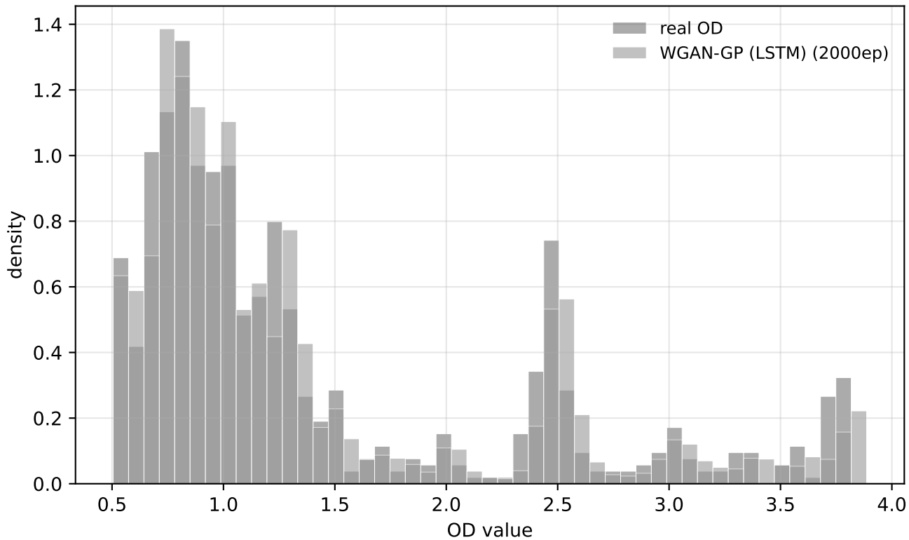
Distribution comparison — WGAN-GP (LSTM)
