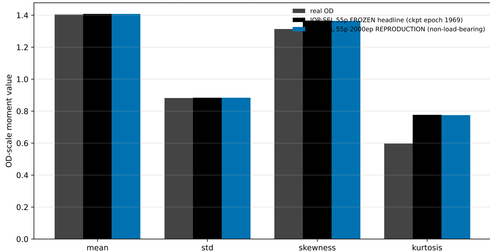
Frozen headline vs 2000ep reproduction (55-param IQP:SEL) — labelled DISTINCTLY (D-14-10)
