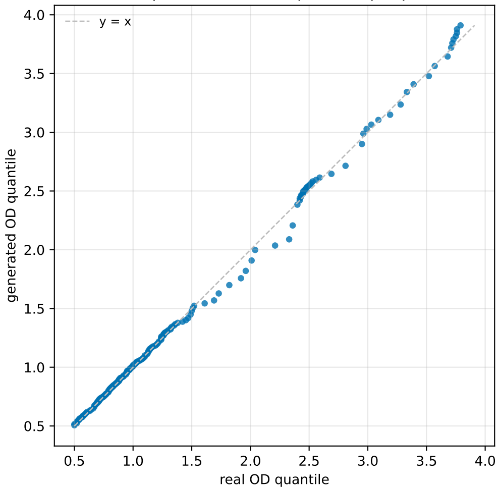
Q-Q plot — IQP:SEL 55p (2000ep repro)
