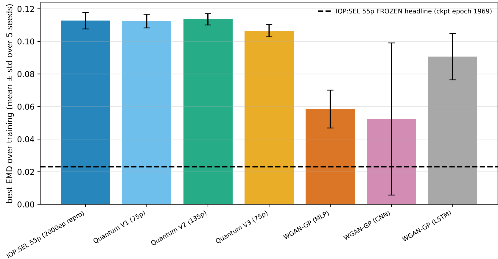
Cross-model EMD (2000ep matched budget)
