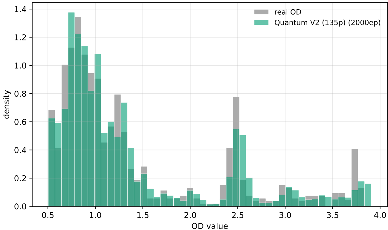
Distribution comparison — Quantum V2 (135p)
