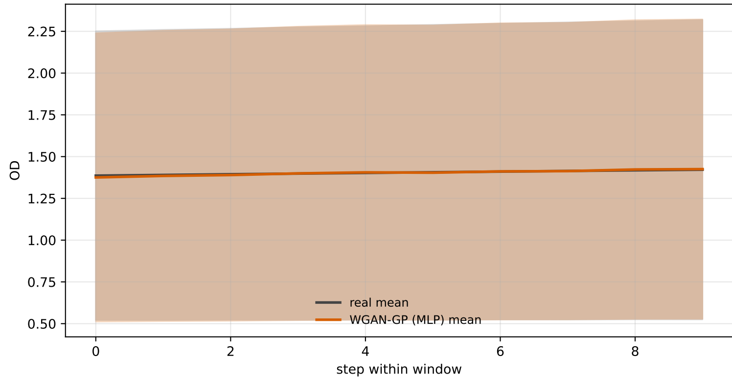
OD reconstruction — WGAN-GP (MLP)
