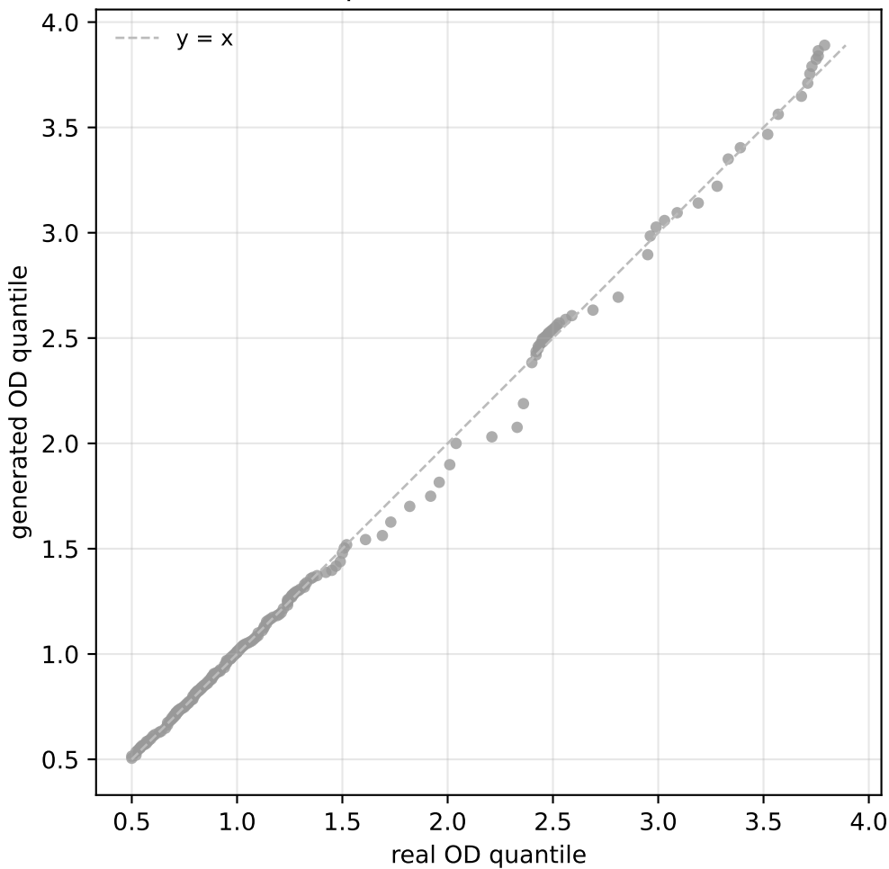
Q-Q plot — WGAN-GP (LSTM)
