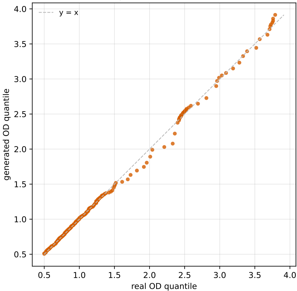
Q-Q plot — WGAN-GP (MLP)
