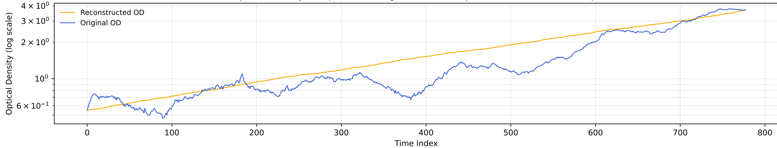
Optical Density Comparison — Log Scale (all 778 points) — Quantum V1 (75p)
