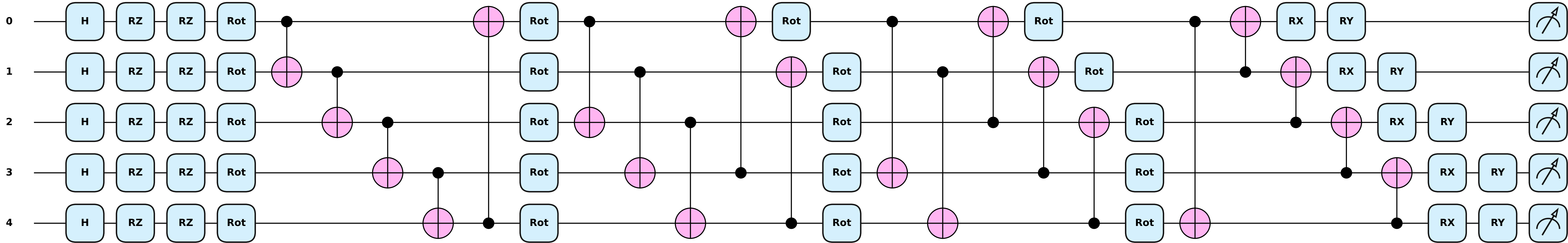
default_75 - 5 qubits x 4 layers x range topology - 75 parameters
