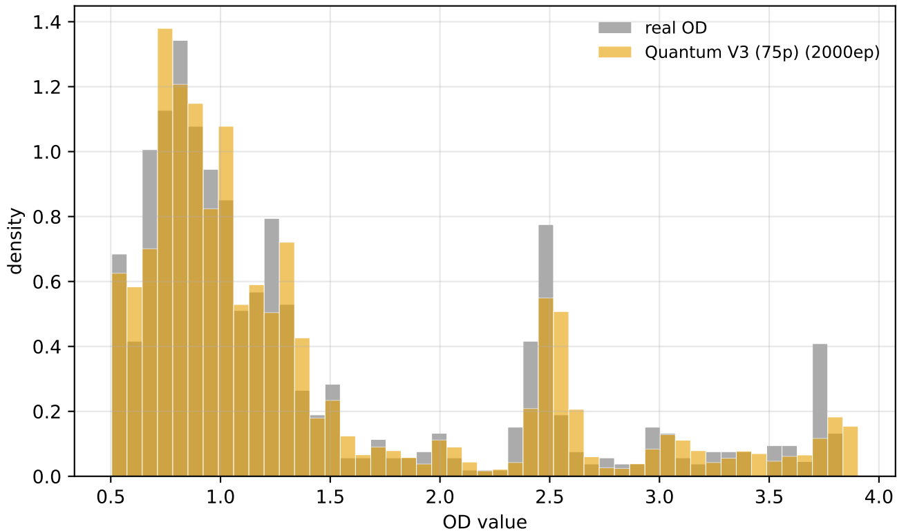
Distribution comparison — Quantum V3 (75p)
