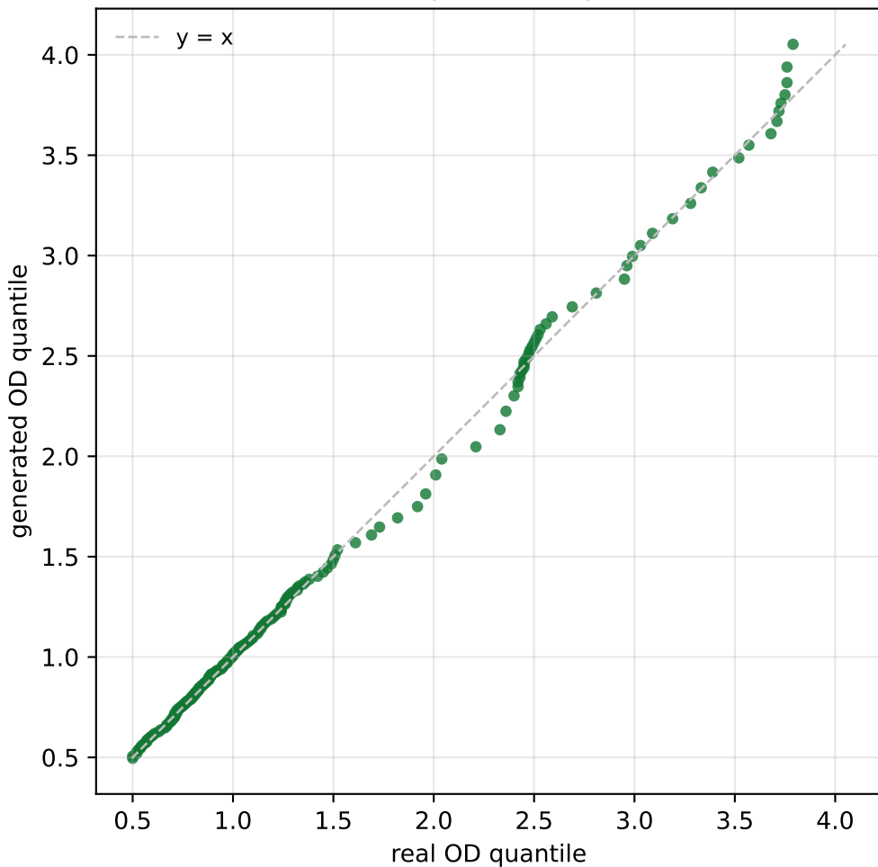
Q-Q plot — AR(p)
