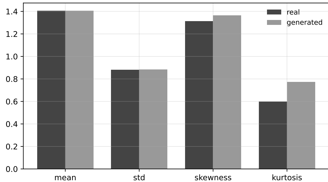
(a) moments
