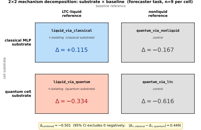
FIG. 17. Schematic of the 2 \times 2 mechanism-decomposition design introduced by amendments A12–A13. Rows index the cell substrate (classical MLP vs. quantum cell); columns index the baseline reference (LTC-liquid vs. nonliquid Neural ODE). Each cell yields a per-cell \Delta_{\text{diff}} ; the four numbers algebraically partition the headline forecaster \Delta_{\text{combined}} = -0.501 into a sum of substrate and reference contributions plus an interaction term. The interaction term is the substrate-dependent \tau signature analyzed in Figure 18.
