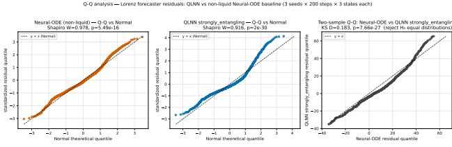
FIG. 9. Q-Q residual diagnostic on the Lorenz forecaster cell. Left : non-liquid Neural-ODE residuals vs standard Normal, Shapiro W=0.978 , p=5.5 \times 10^{-16} . Middle : QLNN strongly-entangling residuals vs standard Normal, W=0.916 , p=2.0 \times 10^{-30} — pronounced S-shape with heavy right tail. Right : two-sample Q-Q of the two empirical distributions, Kolmogorov–Smirnov D=0.183 , p=7.7 \times 10^{-27} — distributions are distinguishable at very high significance, and the points depart systematically from y=x in the upper tail (the QLNN’s worst-case residuals are markedly larger). Built via the reusable _qq_panel_vs_normal and _two_sample_qq helpers added in Amendment A14; the harness is dataset-agnostic and applies unchanged to any other (model, system) cell with on-disk field.npz artifacts.
