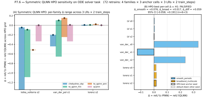
FIG. 12. Symmetric HPO sensitivity (P7.6 amendment A9): both sides tuned at three anchor cells across three learning rates and two training-step budgets. The HPO-best n = 9 verdict (Table VI, row 4) is FALSIFIED with point estimate +0.059 and CI [-0.058, +0.191] , methodologically strengthening the default-Adam n = 18 row directly above it.
