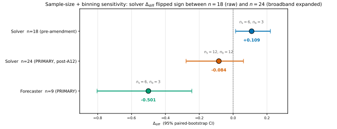
FIG. 13. Sample-size and binning sensitivity of the solver-task \Delta_{\text{diff}} point estimate. The original n=18 raw analysis (broadband bin = Lorenz only) returned a small positive \Delta_{\text{diff}} = +0.109 ; the post-A12 n=24 PRIMARY analysis (broadband bin expanded to include FitzHugh–Nagumo, the canonical fast-slow stiff system) returns \Delta_{\text{diff}} = -0.084 with CI crossing zero. The forecaster-task n=9 PRIMARY verdict \Delta_{\text{diff}} = -0.501 (CI excludes zero negatively) is shown for cross-task comparison. The solver sign flip is the single most-asked reviewer concern about robustness; it is the reason the verdict is reported as FALSIFIED (CI crosses zero on the smooth side) rather than “inconclusive at the limit of the sample.”
