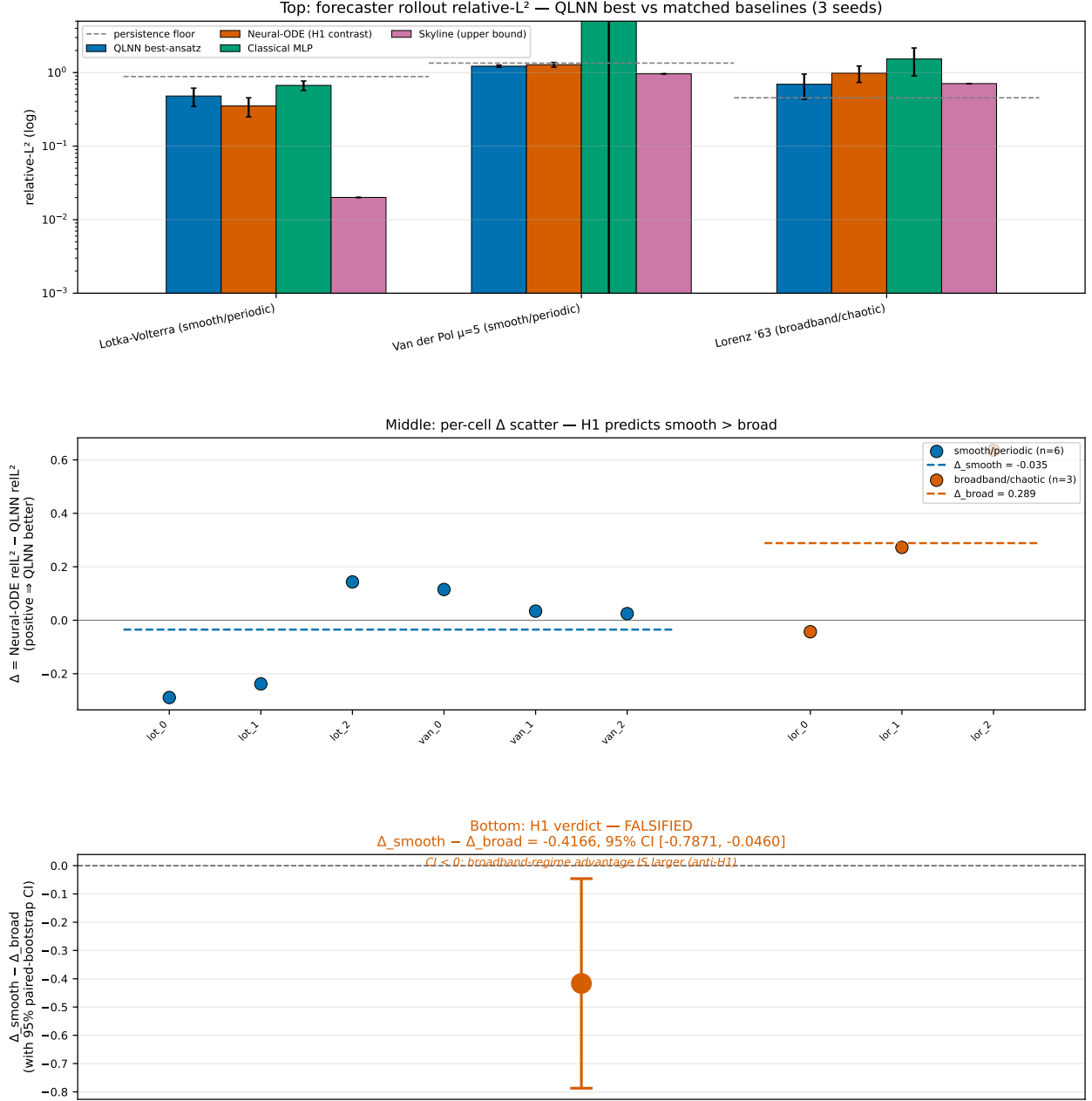
FIG. 11. Pre-registered H_1 forecaster verdict at the original P_5 configuration ( n = 6 post-guard, retained as a layered sensitivity point in Table VI; the PRIMARY forecaster verdict that replaces this row is the P_{7.10} row \Delta_{\text{diff}} = -0.501 at n = 9 ). Top: per-system relative- L^2 for QLNN best vs. matched Neural-ODE, MLP, known-structure skyline, and persistence floor across the three smooth/periodic and three broadband/chaotic systems of the hardness ladder. Middle: per-cell \Delta = \text{Neural-ODE} - \text{QLNN} stratified by regime (blue: smooth/periodic, \bar{\Delta}_{\text{smooth}} = -0.128 ; orange: broadband/chaotic, \bar{\Delta}_{\text{broad}} = +0.289 ). Bottom: the test statistic \Delta_{\text{smooth}} - \Delta_{\text{broad}} = -0.417 with paired-bootstrap 95% CI [-0.787, -0.046] over n = 6 post-guard cells. The CI excludes zero in the negative direction; per pre-registration §7, the verdict is FALSIFIED on the matched-capacity forecaster contrast. Source: results/p5_h1_verdict/h1_analysis.json .
