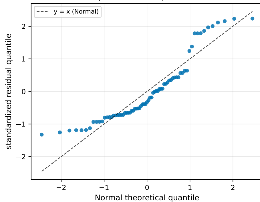
QLNN 4q/3L — Q-Q vs Normal Shapiro W=0.885, p=8.91e-06
