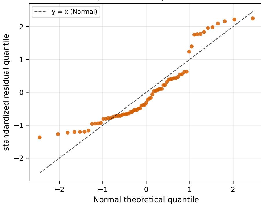
Classical H=4 — Q-Q vs Normal Shapiro W=0.892, p=1.64e-05
