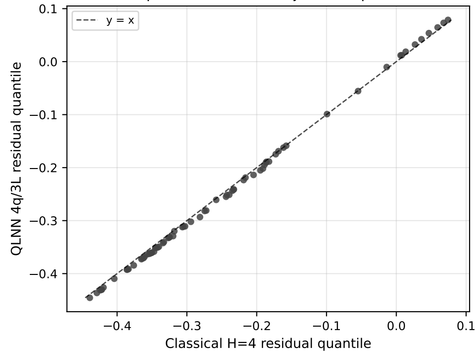
Two-sample Q-Q: Classical H=4 vs QLNN 4q/3L KS D=0.085, p=0.964 (cannot reject H_0 equal distributions)
