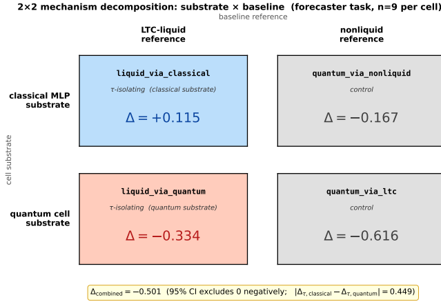
FIG. 10. Schematic of the 2x2 mechanism-decomposition design introduced by amendments A12–A13. Rows index the cell substrate (classical MLP vs. quantum cell); columns index the baseline reference (LTC-liquid vs. nonliquid Neural-ODE). Each cell yields a per-cell \Delta_{\text{diff}} ; the four numbers algebraically partition the headline forecaster \Delta_{\text{combined}} = -0.501 into a sum of substrate and reference contributions plus an interaction term. The interaction term is the substrate-dependent \tau signature analyzed in Figure 11.
