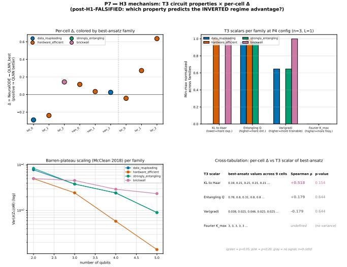
FIG. 12. KL-to-Haar expressivity distance is the only trainability scalar with sign-stable correlation to per-cell performance; all 9 leave-one-out resamples remain positive. H_3 mechanism cross-tabulation: per-family T3 scalars (Meyer–Wallach Q , KL-to-Haar divergence, gradient variance, Fourier K_{\text{max}} ) versus per-cell \Delta on the forecaster task. KL-to-Haar (lower = more expressive) is the only scalar with a sign-stable leave-one-out trend ( \rho = +0.518 , all 9 LOO resamples positive).
