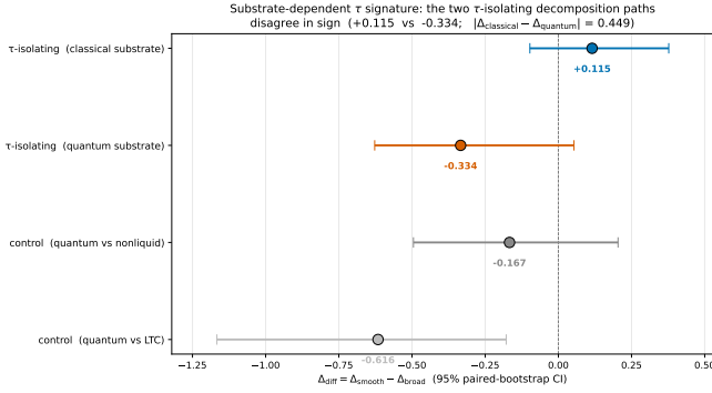
FIG. 11. Substrate-dependent \tau signature: the two decomposition paths that isolate the liquid time-constant machinery ( liquid_via_classical , liquid_via_quantum ) disagree in sign, with |\Delta_{\text{classical}} - \Delta_{\text{quantum}}| \approx 0.449 . The two control paths ( quantum_via_ltc , quantum_via_nonliquid ), which do not isolate \tau , are both negative and broadly consistent with the combined verdict. This pattern is the strongest mechanistic evidence in the paper that LTC-style time-constant machinery interacts with the substrate it is mounted on, and is the seed for a planned follow-up paper (Section VII).
