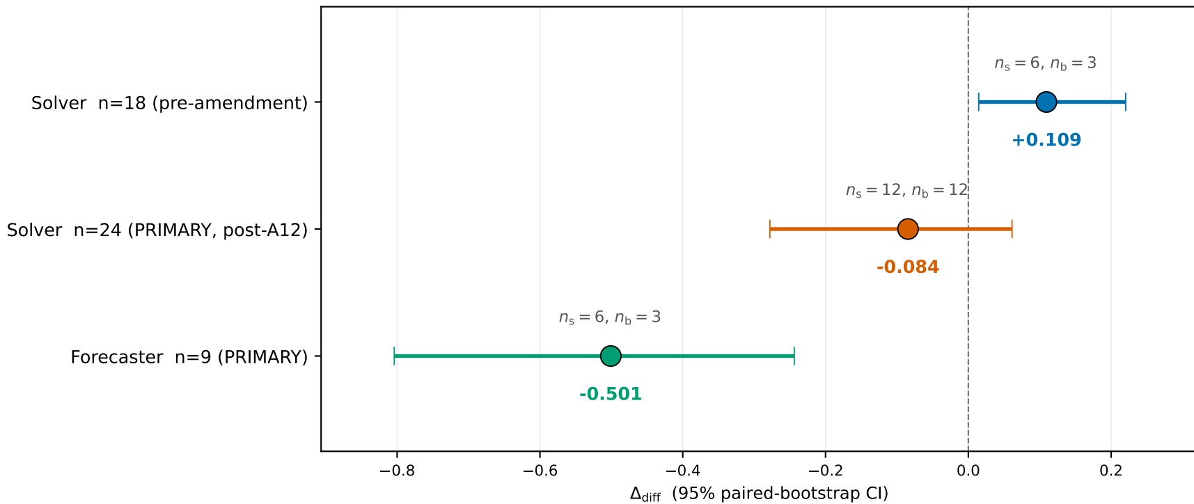
Sample-size + binning sensitivity: solver \Delta_{\text{diff}} flipped sign between n = 18 (raw) and n = 24 (broadband expanded)
