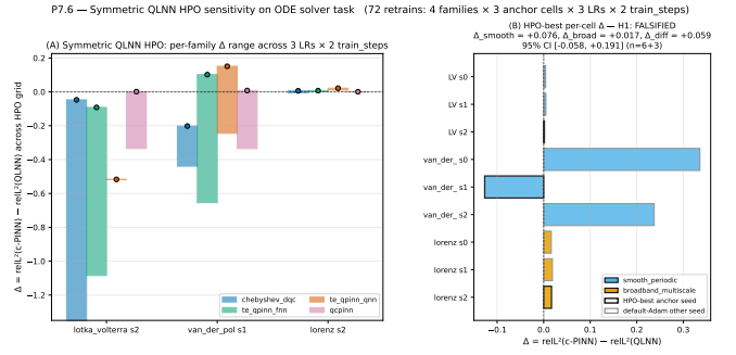
FIG. 7. Symmetric HPO sensitivity (P7.6 amendment A9): both sides tuned at three anchor cells across three learning rates and two training-step budgets. The HPO-best n = 9 verdict (Table VI, row 4) is FALSIFIED with point estimate +0.059 and CI [-0.058, +0.191] , methodologically strengthening the default-Adam n = 18 row directly above it.
