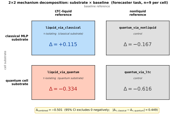
FIG. 10. Schematic of the 2x2 mechanism-decomposition design introduced by amendments A12–A13. Rows index the cell substrate (classical MLP vs. quantum cell); columns index the baseline reference (LTC-liquid vs. nonliquid Neural-ODE). Each cell yields a per-cell \Delta_{\text{diff}} ; the four numbers algebraically partition the headline forecaster \Delta_{\text{combined}} = -0.501 into a sum of substrate and reference contributions plus an interaction term. The interaction term is the substrate-dependent \tau signature analyzed in Figure 11.
