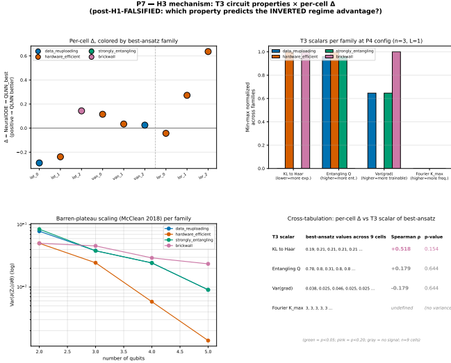
FIG. 12. KL-to-Haar expressivity distance is the only trainability scalar with sign-stable correlation to per-cell performance; all 9 leave-one-out resamples remain positive. H_3 mechanism cross-tabulation: per-family T3 scalars (Meyer-Wallach Q , KL-to-Haar divergence, gradient variance, Fourier K_{\max} ) versus per-cell \Delta on the forecaster task. KL-to-Haar (lower = more expressive) is the only scalar with a sign-stable leave-one-out trend ( \rho = +0.518 , all 9 LOO resamples positive).
