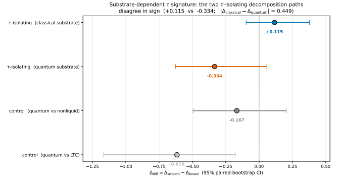
FIG. 11. Substrate-dependent \tau signature: the two decomposition paths that isolate the liquid time-constant machinery ( liquid_via_classical , liquid_via_quantum ) disagree in sign, with |\Delta_{\text{classical}} - \Delta_{\text{quantum}}| \approx 0.449 . The two control paths ( quantum_via_ltc , quantum_via_nonliquid ), which do not isolate \tau , are both negative and broadly consistent with the combined verdict. This pattern is the strongest mechanistic evidence in the paper that LTC-style time-constant machinery interacts with the substrate it is mounted on, and is the seed for a planned follow-up paper (Section VII).
