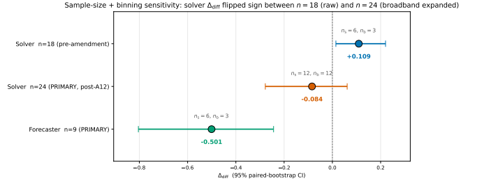
FIG. 8. Sample-size and binning sensitivity of the solver-task \Delta_{\text{diff}} point estimate. The original n=18 raw analysis (broadband bin = Lorenz only) returned a small positive \Delta_{\text{diff}} = +0.109 ; the post-A12 n=24 PRIMARY analysis (broadband bin expanded to include FitzHugh–Nagumo, the canonical fast-slow stiff system) returns \Delta_{\text{diff}} = -0.084 with CI crossing zero. The forecaster-task n=9 PRIMARY verdict \Delta_{\text{diff}} = -0.501 (CI excludes zero negatively) is shown for cross-task comparison. The solver sign flip is the single most-asked reviewer concern about robustness; it is the reason the verdict is reported as FALSIFIED (CI crosses zero on the smooth side) rather than “inconclusive at the limit of the sample.”
