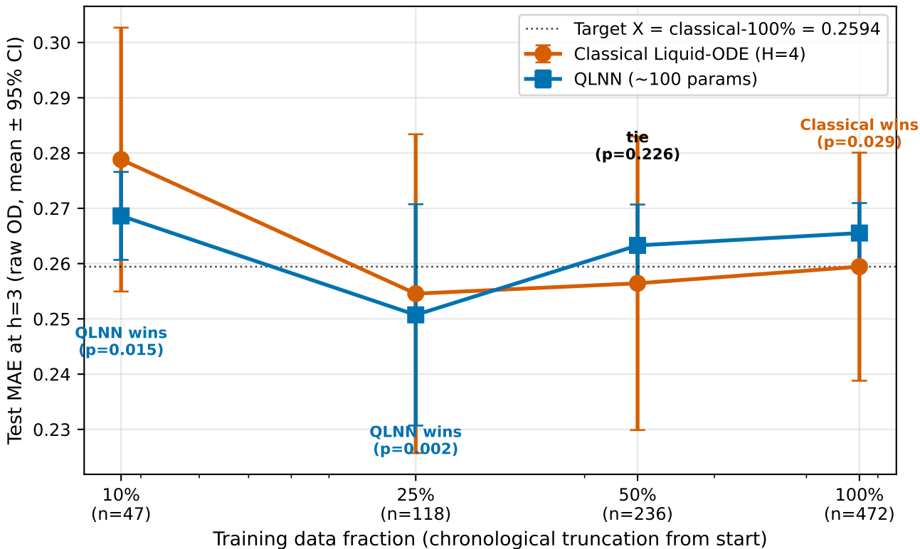
Sample-efficiency crossover at h=3 (paired-bootstrap verdicts shown)
