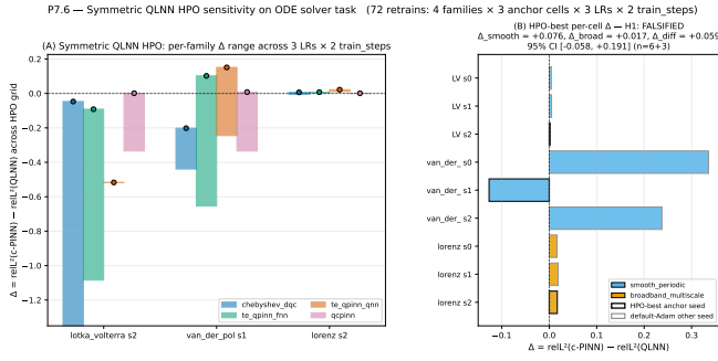
FIG. 12. Symmetric HPO sensitivity (P7.6 amendment A9): both sides tuned at three anchor cells across three learning rates and two training-step budgets. The HPO-best n = 9 verdict (Table VI, row 4) is FALSIFIED with point estimate +0.059 and CI [-0.058, +0.191] , methodologically strengthening the default-Adam n = 18 row directly above it.
