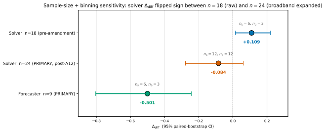
FIG. 13. Sample-size and binning sensitivity of the solver-task \Delta_{\text{diff}} point estimate. The original n=18 raw analysis (broadband bin = Lorenz only) returned a small positive \Delta_{\text{diff}} = +0.109 ; the post-A12 n=24 PRIMARY analysis (broadband bin expanded to include FitzHugh–Nagumo, the canonical fast-slow stiff system) returns \Delta_{\text{diff}} = -0.084 with CI crossing zero. The forecaster-task n=9 PRIMARY verdict \Delta_{\text{diff}} = -0.501 (CI excludes zero negatively) is shown for cross-task comparison. The solver sign flip is the single most-asked reviewer concern about robustness; it is the reason the verdict is reported as FALSIFIED (CI crosses zero on the smooth side) rather than “inconclusive at the limit of the sample.”
