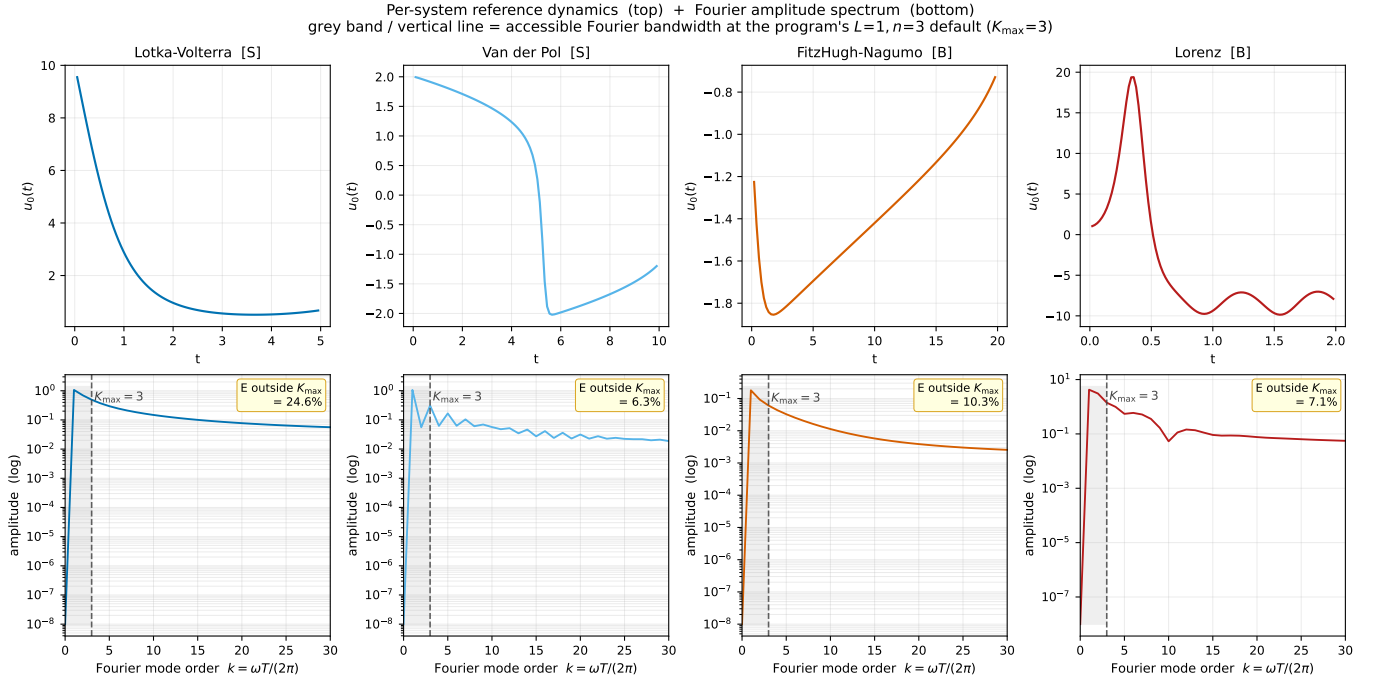
FIG. 6. Per-system Fourier amplitude spectrum (bottom row) plotted on the same Fourier-mode-order axis k = \omega T/(2\pi) so that K_{\max} at the program's default L=1, n=3 chebyshev-DQC configuration sits at x=3 in every panel (grey vertical line and shaded band). Reference trajectories shown in the top row for context (first state component, seed 0). The fraction of spectral energy lying outside the accessible bandwidth is annotated per panel. The figure shows that all four systems concentrate the bulk of their spectral energy in the k \leq 3 band, which is consistent with the H3 cross-tabulation finding that K_{\max} alone (held at the theoretical ceiling K_{\max} = L \cdot n = 3 uniformly across families) does not discriminate among families at this configuration. The broadband/multiscale character of FHN and Lorenz that drives the H1 verdict (Section V) is a structural feature of the dynamics (chaoticity, stiffness, sharp transitions) that the bare Fourier spectrum does not fully expose.
