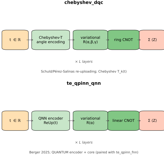
FIG. 5. Schematic of the four quantum ansatz families on the solver-task surface. Each family combines (i) a real-valued time input, (ii) an encoding stage, (iii) a variational stage with single-qubit rotations, (iv) an entanglement stage, and (v) a Pauli-Z readout. The families differ in which stages are classical versus quantum: chebyshev_dqc uses a Chebyshev- T angle encoding plus a ring-CNOT topology; the paired te_qpinn_fnn / te_qpinn_qnn families differ only in whether the encoder is a classical FNN or a quantum re-uploading block; qcpinn (Sedykh et al. 2024) wraps a quantum block in classical pre- and post-nets, and amendment A17 sweeps the quantum-to-classical parameter ratio across three additional variants qcpinn_balanced , qcpinn_quantum , and qcpinn_full_q ( Q/(Q+C) \approx 24\%, 45\%, 87\% respectively).
