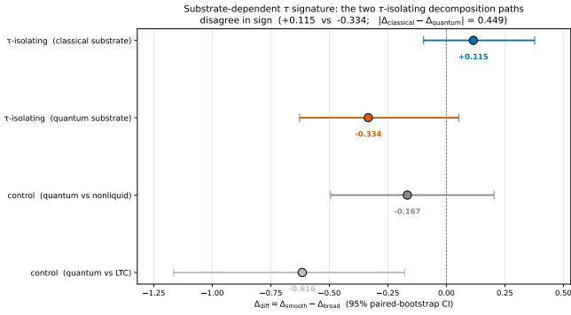
FIG. 18. Substrate-dependent \tau signature: the two decomposition paths that isolate the liquid time-constant machinery ( liquid.via.classical , liquid.via.quantum ) disagree in sign, with |\Delta_{\text{classical}} - \Delta_{\text{quantum}}| \approx 0.449 . The two control paths ( quantum.via.ltc , quantum.via.nonliquid ), which do not isolate \tau , are both negative and broadly consistent with the combined verdict. This pattern is the strongest mechanistic evidence in the paper that LTC-style time-constant machinery interacts with the substrate it is mounted on, and is the seed for a planned follow-up paper (Section VII).
