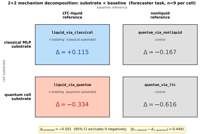
FIG. 17. Schematic of the 2 \times 2 mechanism-decomposition design introduced by amendments A12–A13. Rows index the cell substrate (classical MLP vs. quantum cell); columns index the baseline reference (LTC-liquid vs. nonliquid Neural-ODE). Each cell yields a per-cell \Delta_{\text{diff}} ; the four numbers algebraically partition the headline forecaster \Delta_{\text{combined}} = -0.501 into a sum of substrate and reference contributions plus an interaction term. The interaction term is the substrate-dependent \tau signature analyzed in Figure 18.
