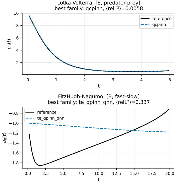
FIG. 7. Per-system QLNN-prediction-vs-reference trajectories (seed 0, first state component) for the best-performing quantum family per system at the P3.6 multi-state configuration. Tracking is qualitatively correct on the smooth-periodic regime (Lotka–Volterra, Van der Pol) and degrades systematically on the broadband-multiscale regime (FitzHugh–Nagumo, Lorenz), foreshadowing the per-regime \Delta contrasts that drive the H1 verdict in Section V.
