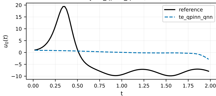
Lorenz [B, chaotic] best family: te_qpinn_qnn, \langle \text{relL}^2 \rangle = 0.978
