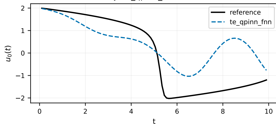
Van der Pol [S, limit cycle] best family: te_qpinn_fnn, \langle \text{relL}^2 \rangle = 0.835
