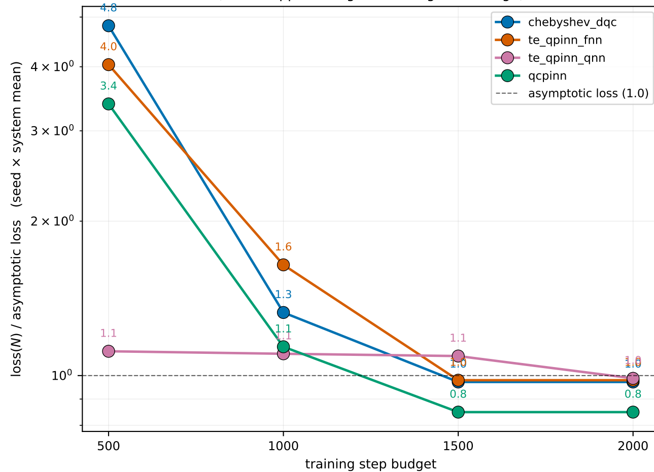
Convergence ratio across the 4 ODE solver families (values approaching 1.0 = budget is enough)
