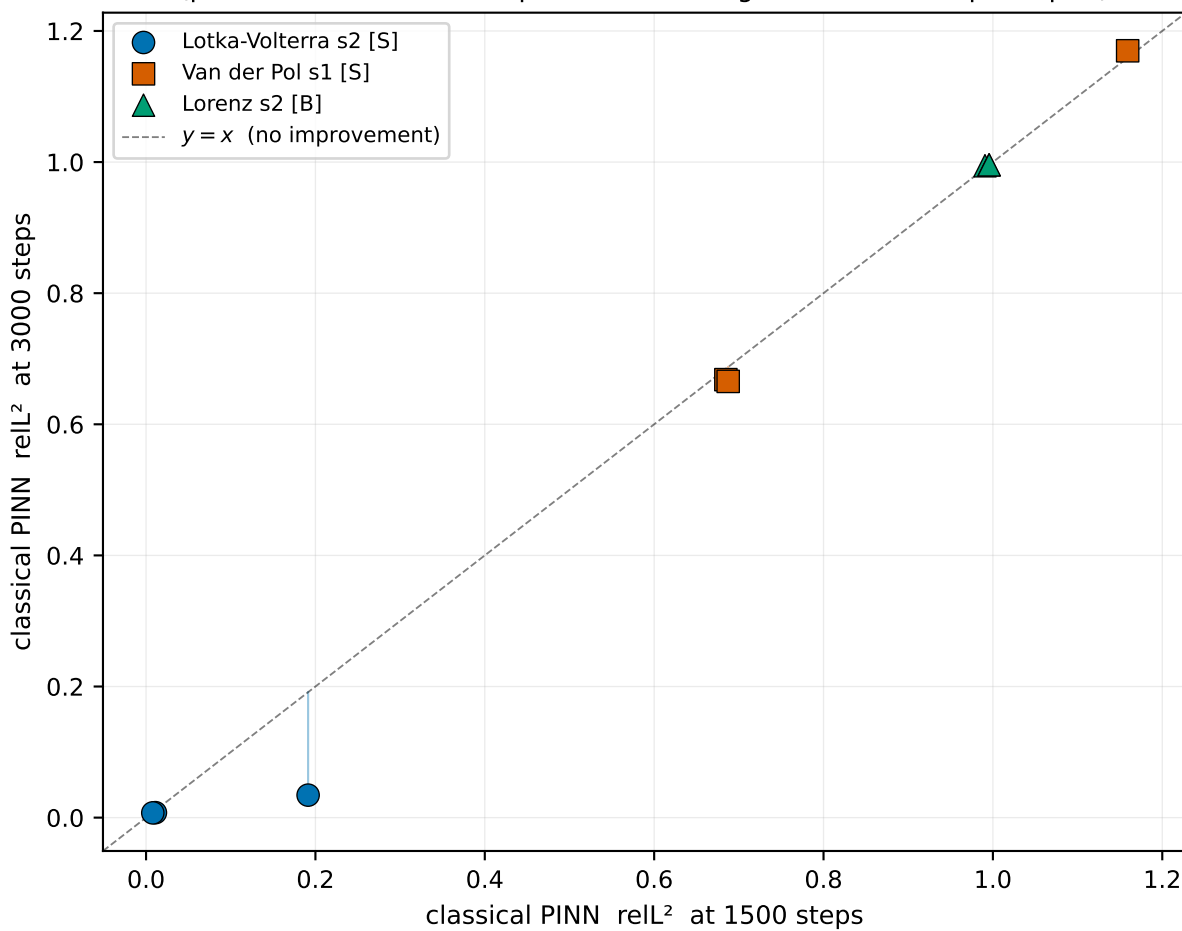
Cross-step diminishing returns on the cPINN baseline (per anchor cell \times 3 LR; points below diagonal = more steps helped)
