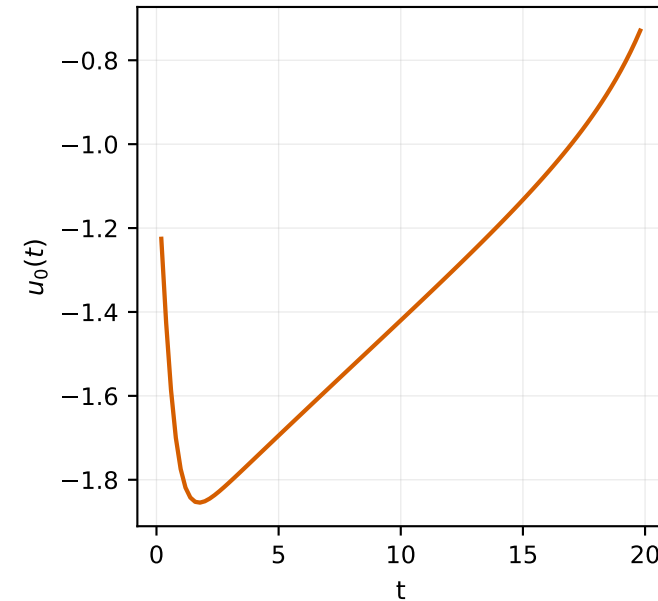
FitzHugh-Nagumo [B]
