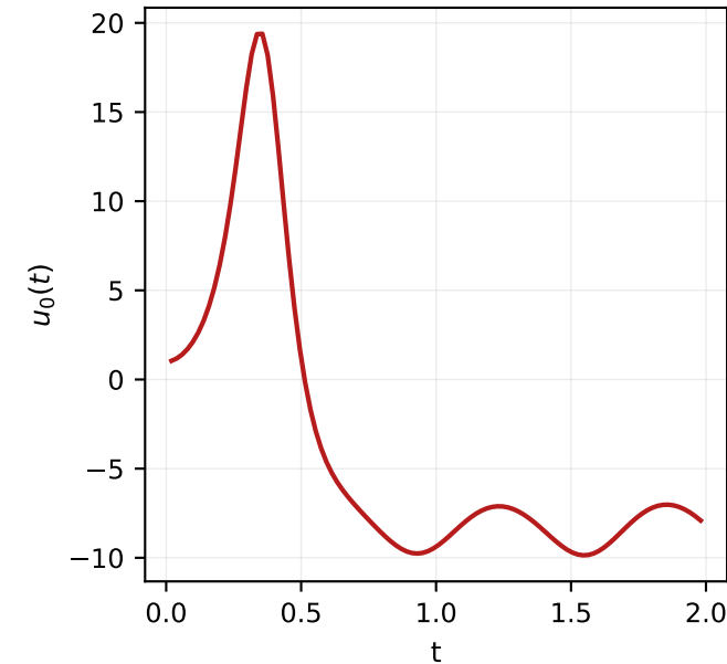
Lorenz [B]
