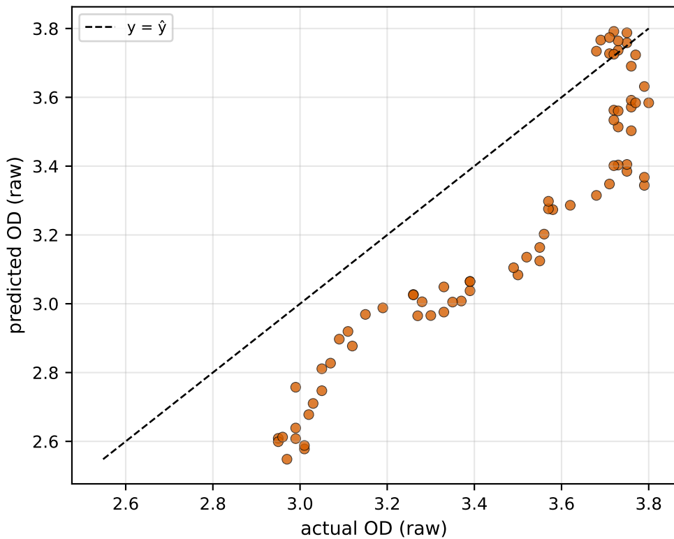
Classical Liquid-ODE (H=4) R^2 = 0.058 (seed-mean prediction)
