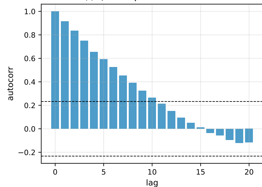
(f) QLNN 4q/3L — residual ACF
