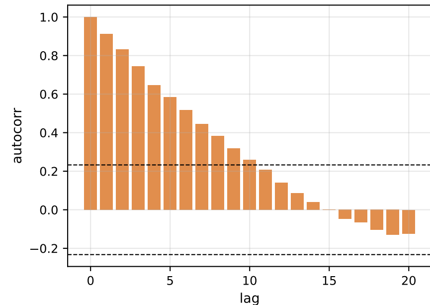
(f) QLNN 4q/3L — residual ACF
