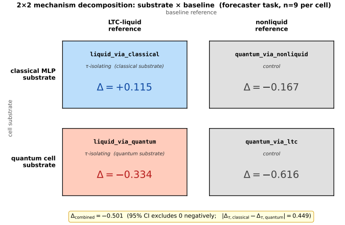
FIG. 17. Schematic of the 2x2 mechanism-decomposition design introduced by amendments A12–A13. Rows index the cell substrate (classical MLP vs. quantum cell); columns index the baseline reference (LTC-liquid vs. nonliquid Neural-ODE). Each cell yields a per-cell \Delta_{\text{diff}} ; the four numbers algebraically partition the headline forecaster \Delta_{\text{combined}} = -0.501 into a sum of substrate and reference contributions plus an interaction term. The interaction term is the substrate-dependent \tau signature analyzed in Figure 18.
