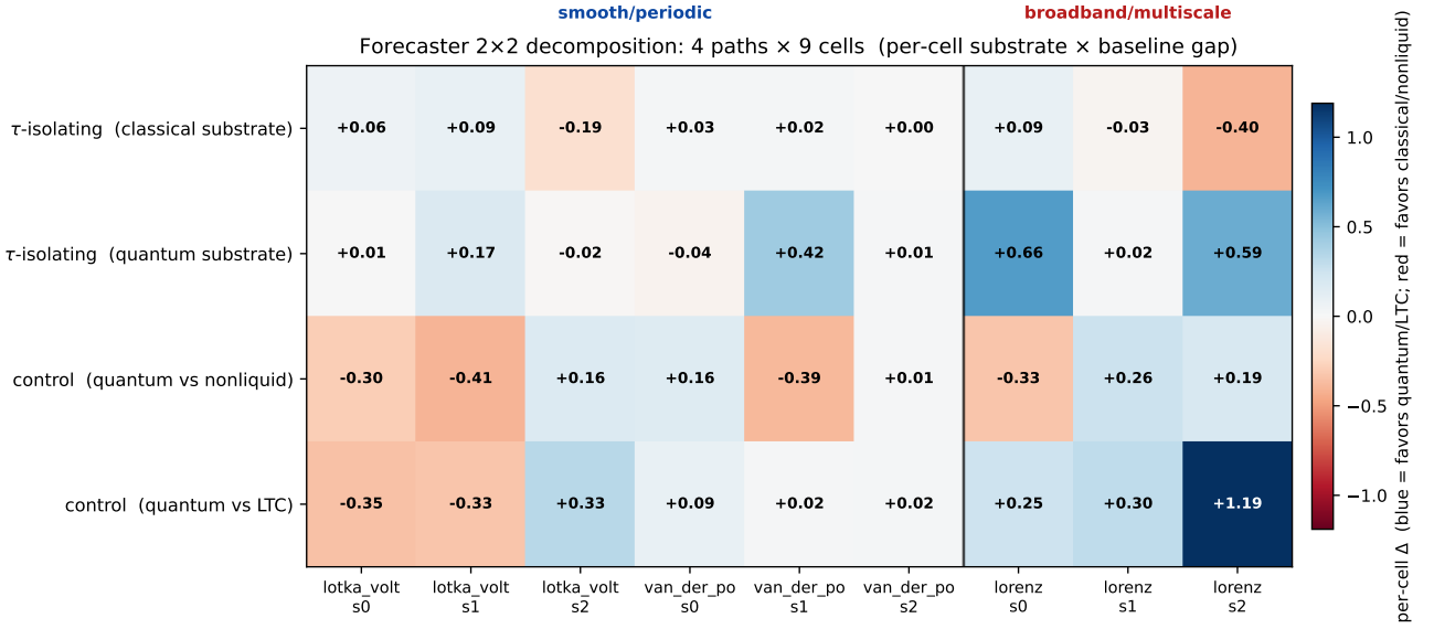
FIG. 20. Forecaster 2x2 decomposition, per-cell breakdown. Rows are the four decomposition paths (Section IV B); columns are the nine (system, seed) cells, with the regime band labeled at the top. Blue cells favor the quantum/LTC side of the contrast; red cells favor the classical/non-liquid side. The substrate-dependent \tau signature (Figure 18) is visible at the per-cell level: the second row (liquid via quantum) carries the strong broadband-positive cells (lorenz s0 = +0.66, lorenz s2 = +0.59), while the controls (rows 3-4) split between negative smooth cells and positive broadband cells, consistent with the -0.501 aggregate verdict and the broadband-leaning sign on the solver task.
