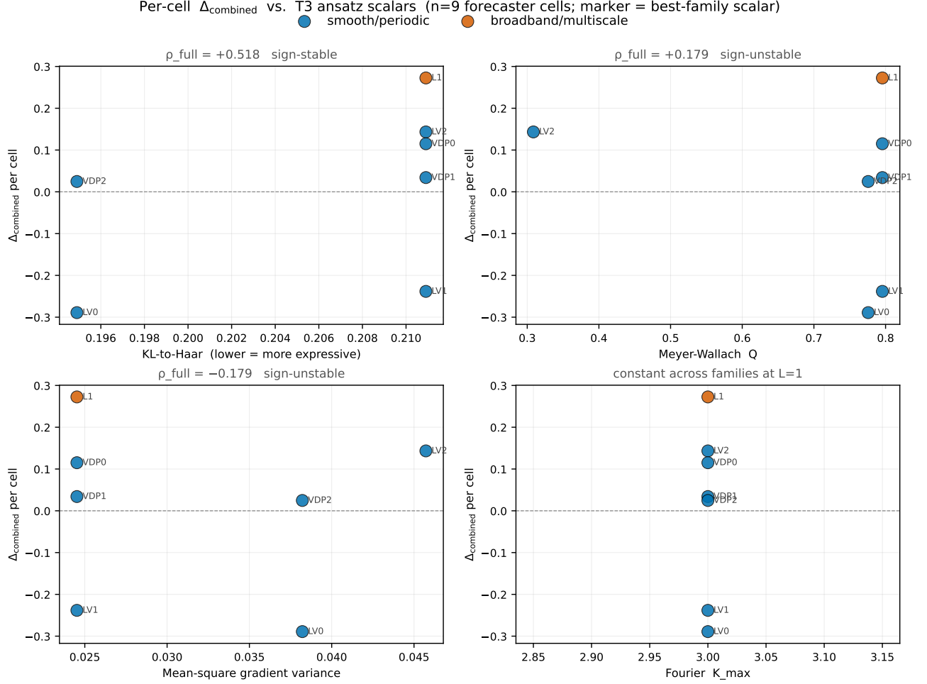
FIG. 19. Per-cell \Delta_{\text{combined}} scattered against each of the four T3 ansatz scalars (KL-to-Haar, Meyer–Wallach Q , mean-square gradient variance, Fourier K_{\max} ) at the cell’s best-quantum family. Color encodes regime (blue = smooth/periodic; orange = broadband/multiscale); marker labels are abbreviated (system, seed). The KL-to-Haar panel (top-left) is the only one with a sign-stable trend ( \rho_{\text{full}} = +0.518 , all-9 LOO resamples positive); Meyer–Wallach Q and gradient variance (top-right, bottom-left) carry weak unstable trends; Fourier K_{\max} (bottom-right) is degenerate at L = 1 . The scatter makes the n=9 sample-size caveat visible: even the sign-stable trend rests on a 9-point spread.
