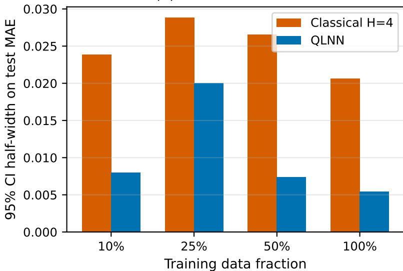
(a) Absolute CI widths
