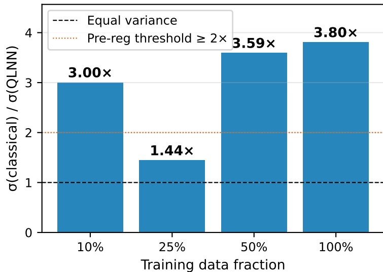
(b) QLNN reproducibility ratio
