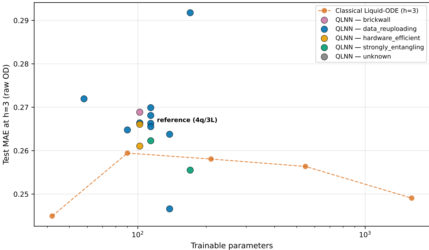
Circuit-search Pareto — QLNN ansatz family vs classical baseline
