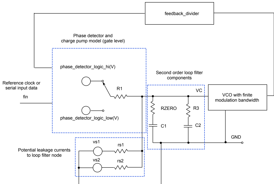
Figure 1 Phase-locked Loop Simulation Program Model
