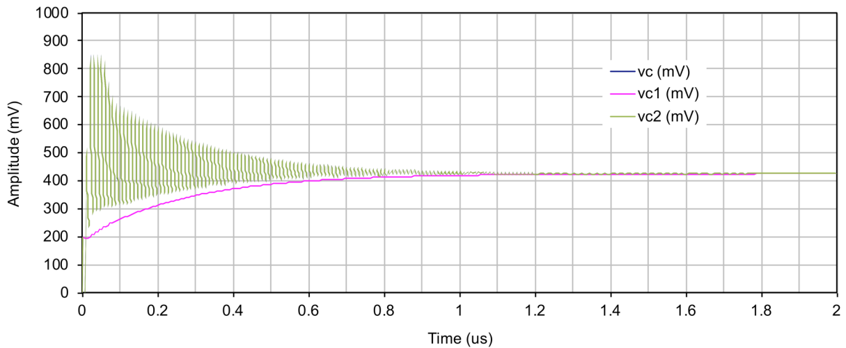
Figure 6 Phase-locked Loop Control Voltage and Loop Filter Capacitor Voltage Variation with Time PFD input frequency = 100.0 MHz, VCO frequency = 12.0 GHz SSC Range = 0 ppm, SSC frequency = 0 kHz
