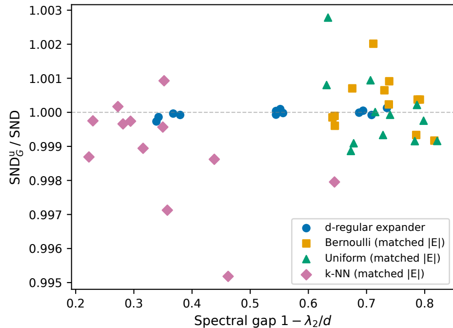
(a) Distortion vs spectral gap
