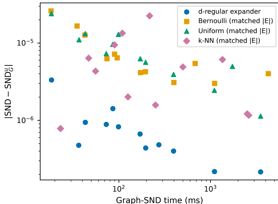
(b) Cost-accuracy Pareto
