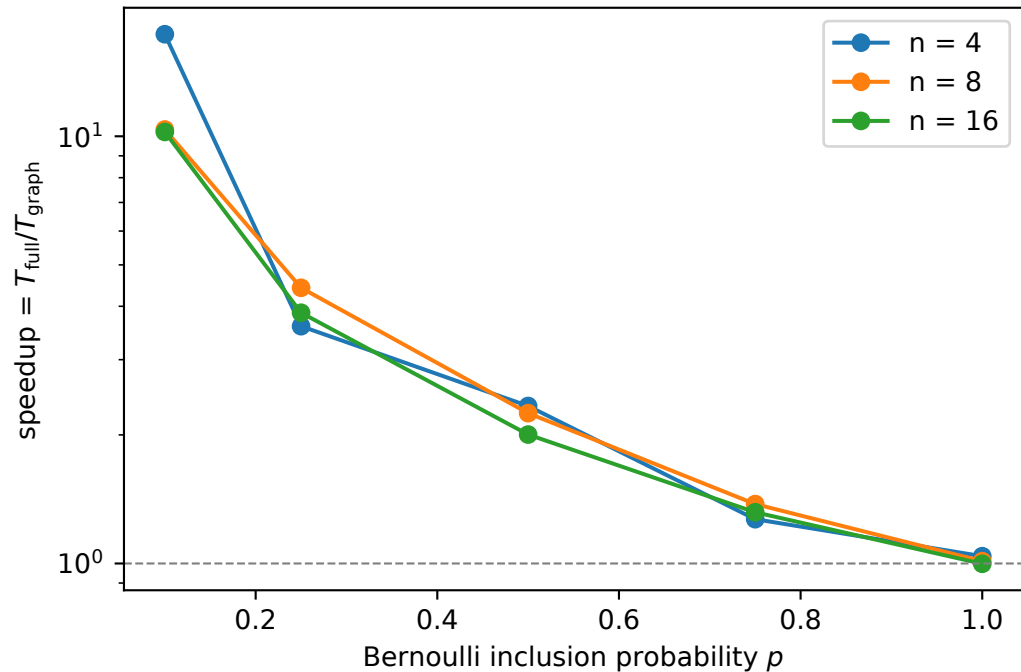
Graph-SND wall-clock speedup
