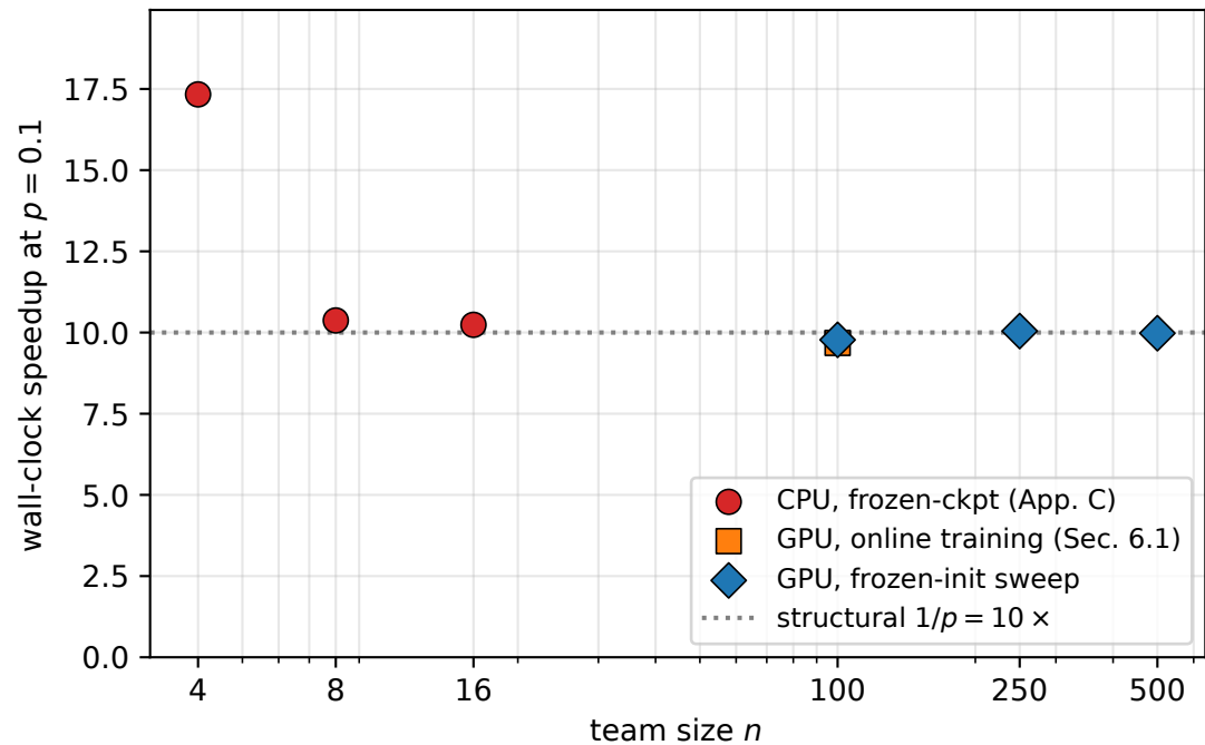
Speedup at p = 0.1 across scale: n \in \{4, 8, 16, 100, 250, 500\}
