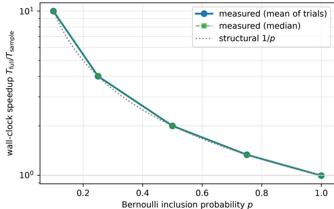
Frozen-init speedup at n = 500 (GPU cuda:0, float32, 20 trials)
