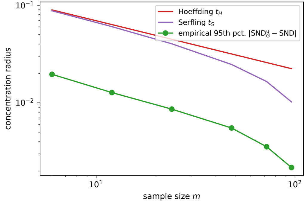
Thm. 9 (n=16, iter100; SND = 0.1073, \delta=0.10 )
