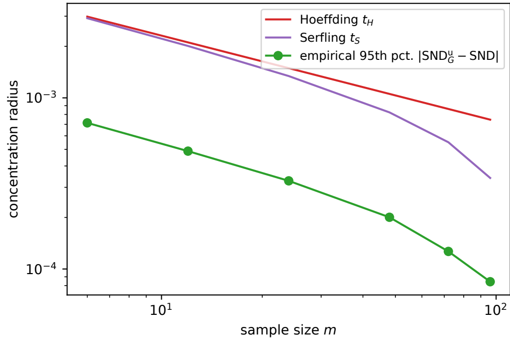
Thm. 9 (n=16, iter0; SND = 0.0031, \delta=0.10 )
