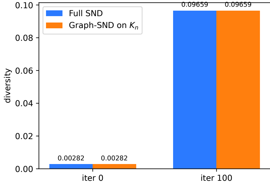
Complete-graph recovery at n = 4
