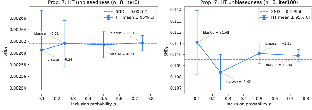
Figure 6: Proposition 7: empirical unbiasedness of \widehat{\text{SND}}_{\text{HT}}(G_p) at n = 8 . Blue dots and whiskers are the sample mean and 95% confidence interval over 2,000 random graphs per p ; the dashed line is the true \text{SND}(\mathbf{D}) . Annotations give the standardized deviation |\text{bias}|/\text{SE} , all of which are well below 1.96. Left: iter 0 checkpoint. Right: iter 100 checkpoint.
