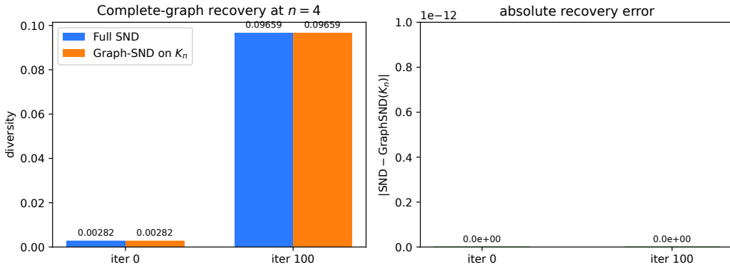
Figure 5: Proposition 2: recovery of SND by \text{SND}_G on the complete graph. Left: side-by-side values of SND and \text{SND}_G on K_4 at iter 0 (near-homogeneous policies) and iter 100 (trained policies). Right: absolute recovery error, which is 0.0 in both cases (the y-axis is shown at 10^{-12} resolution for context).
