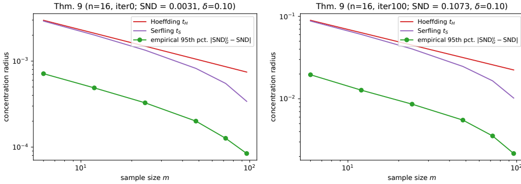
Figure 7: Theorem 9: concentration of \text{SND}_G^u around \text{SND} at n = 16 . Red: Hoeffding radius t_H from Theorem 9. Purple: Serfling radius t_S from Remark 11. Green: empirical 95th-percentile of |\text{SND}_G^u - \text{SND}| over 2,000 uniform-size edge samples per m . Both axes are log-scaled. Across all 12 cells, zero draws violate either bound. The empirical gap reflects the fact that Hoeffding and Serfling are worst-case over populations bounded in [0, D_{\max}] ; the true d(i, j) variance is much smaller.
