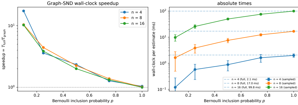
Figure 8: Proposition 6: wall-clock scaling of \text{SND}_G versus SND (CPU, n \in \{4, 8, 16\} ). Left: speedup T_{\text{full}}/T_{\text{sampled}} against Bernoulli inclusion probability p , one line per team size n . Right: absolute wall-clock time per estimate with error bars over 20 trials. Dashed horizontal lines mark the full-SND cost at each n ; solid lines are the sampled \text{SND}_G cost. The red curve in the right panel of Figure 2 plots the p = 0.1 speedups reported here.
