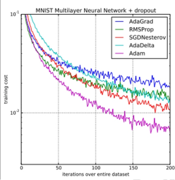
Fig. 7: Cost vs Iterations
