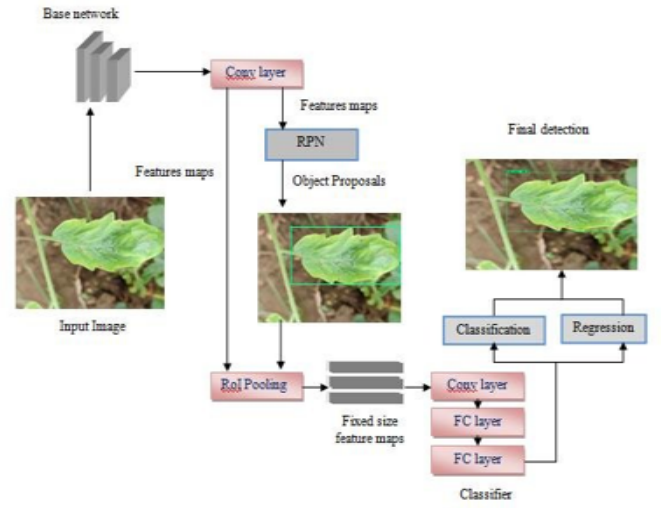
Fig. 11: Disease Detection Flowchart
